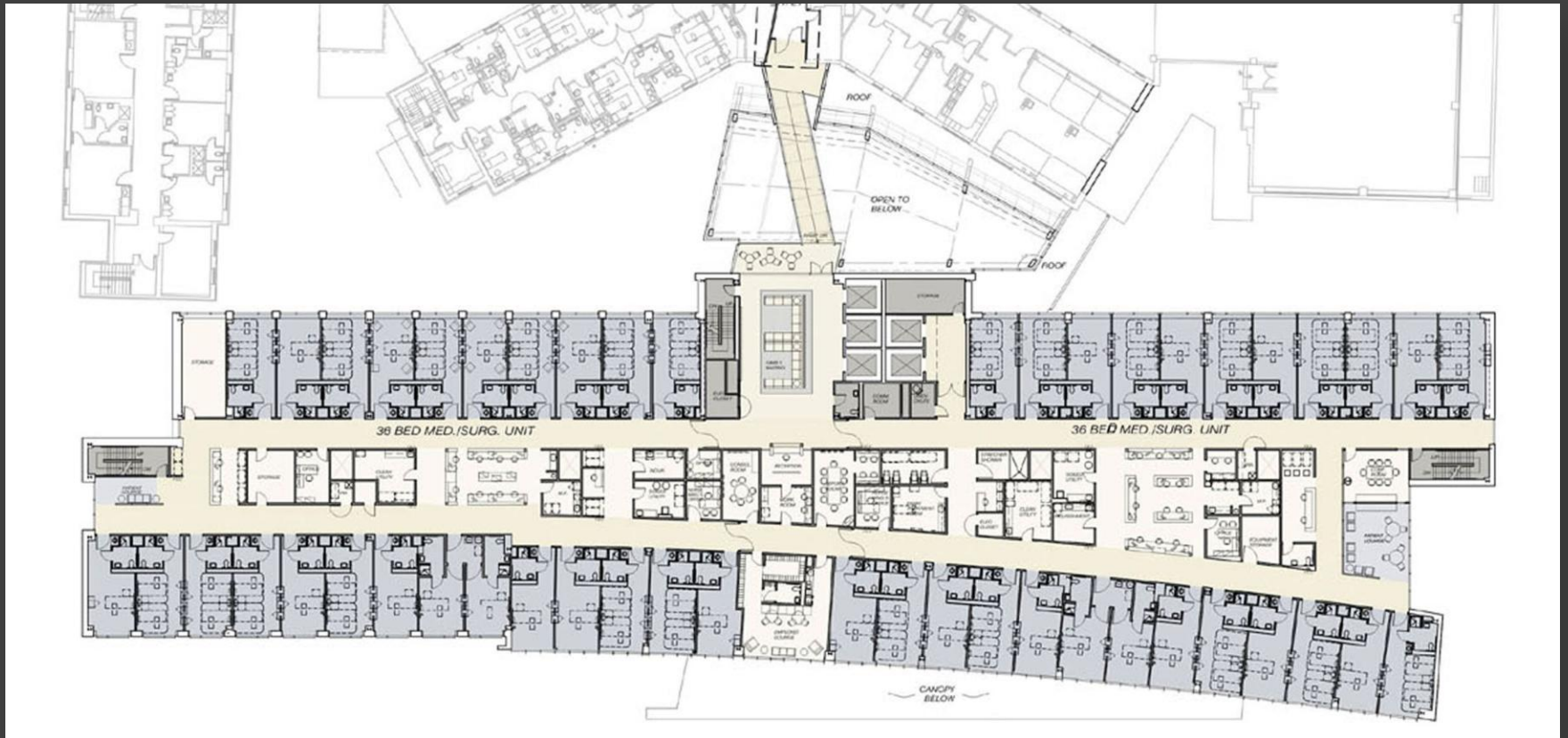
Second Floor
